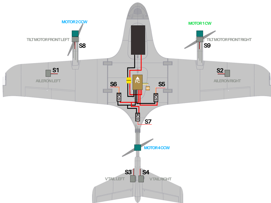
FLIGHTORY STALLION VTOL SAMPLE WIRING DIAGRAM
